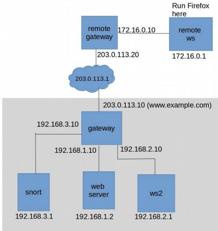
Figure 1: Network topology for the snort lab
